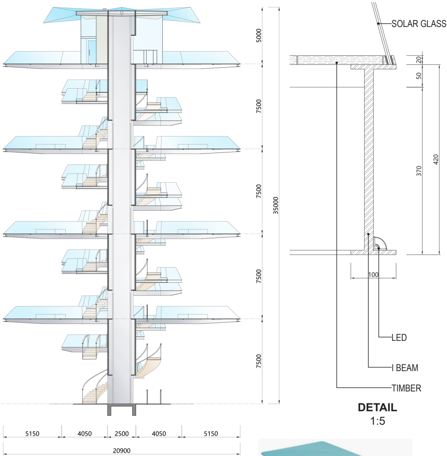
SECTION 1:200
