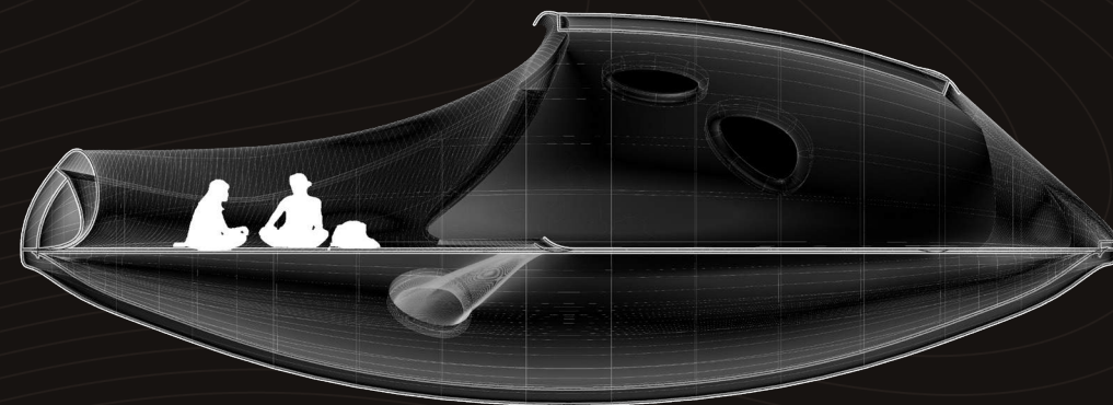
STANDARD LODGE MODULE SECTION | NOT TO SCALE
