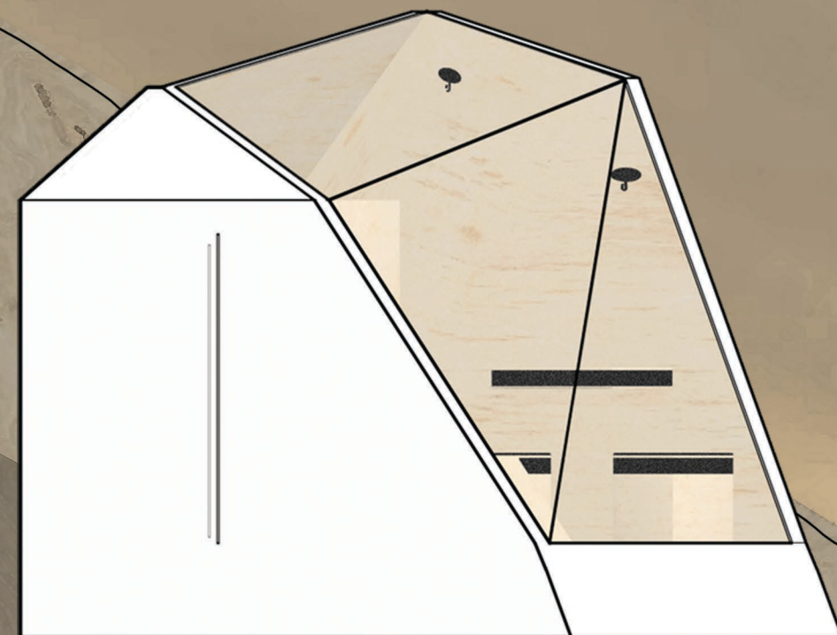
NORTH ELEVATION, SCALE 1:50
