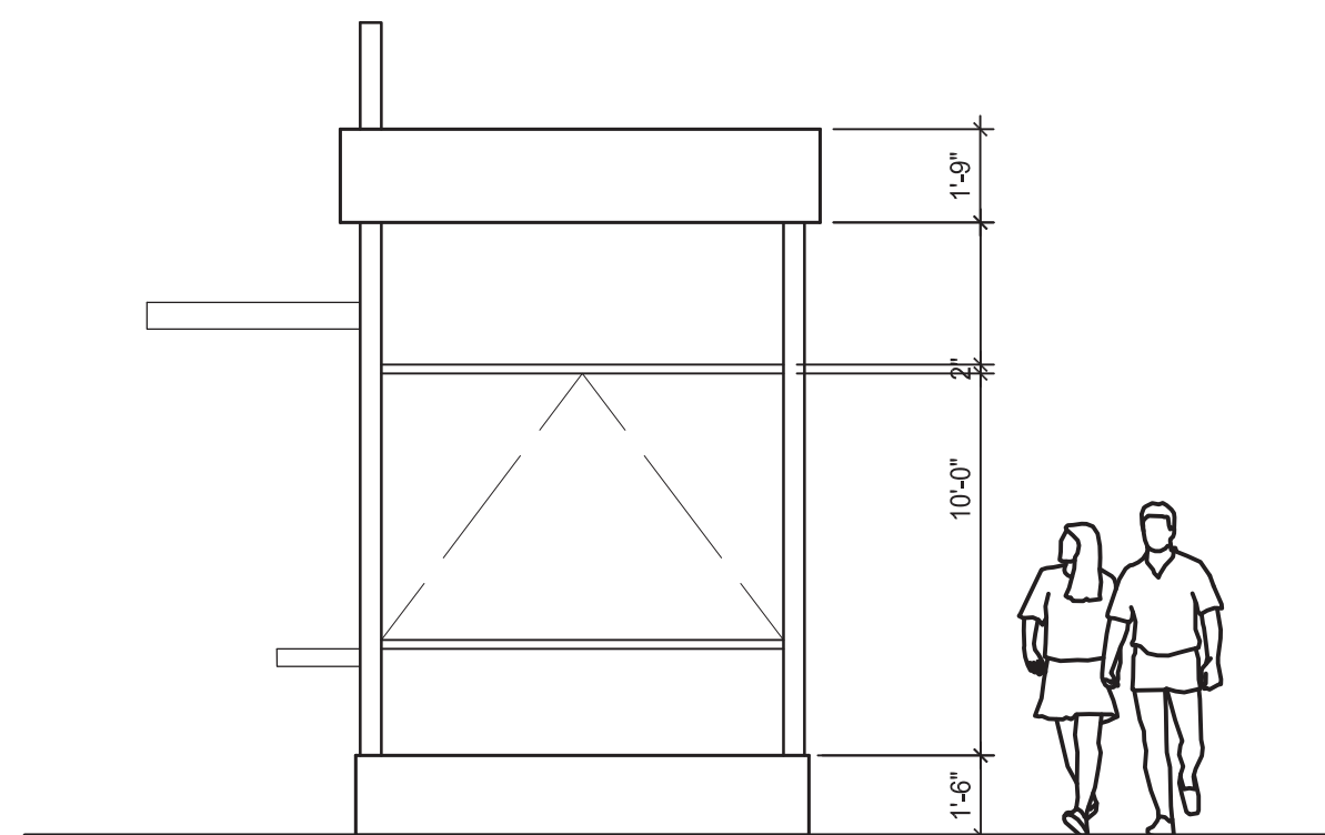
1 EAST EXT. ELEVATION SCALE: 1/4" = 1'-0"
